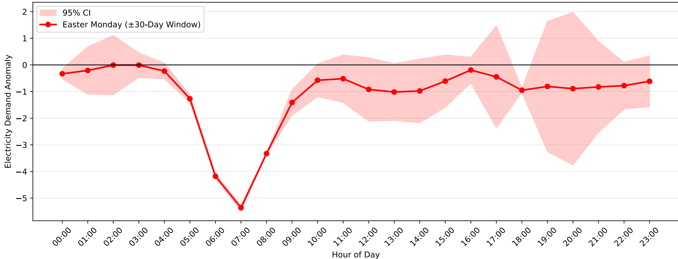
Mortdale Demand Anomaly: Easter Monday (2008-2009, \pm 30 -Day Window)
