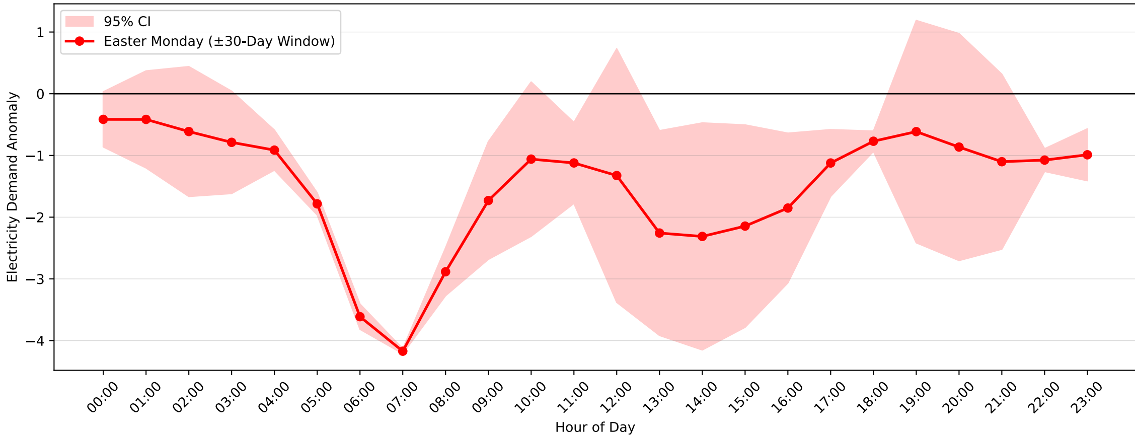
Mortdale Demand Anomaly: Easter Monday (2016-2017, \pm 30 -Day Window)
