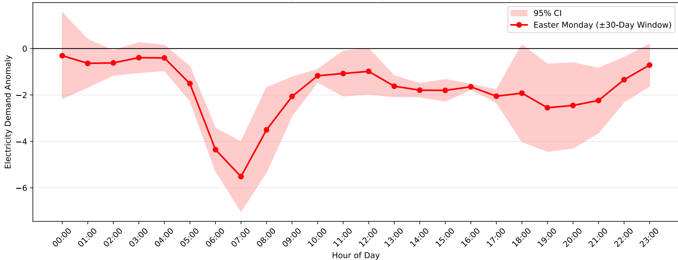
Mortdale Demand Anomaly: Easter Monday (2011-2012, \pm 30 -Day Window)
