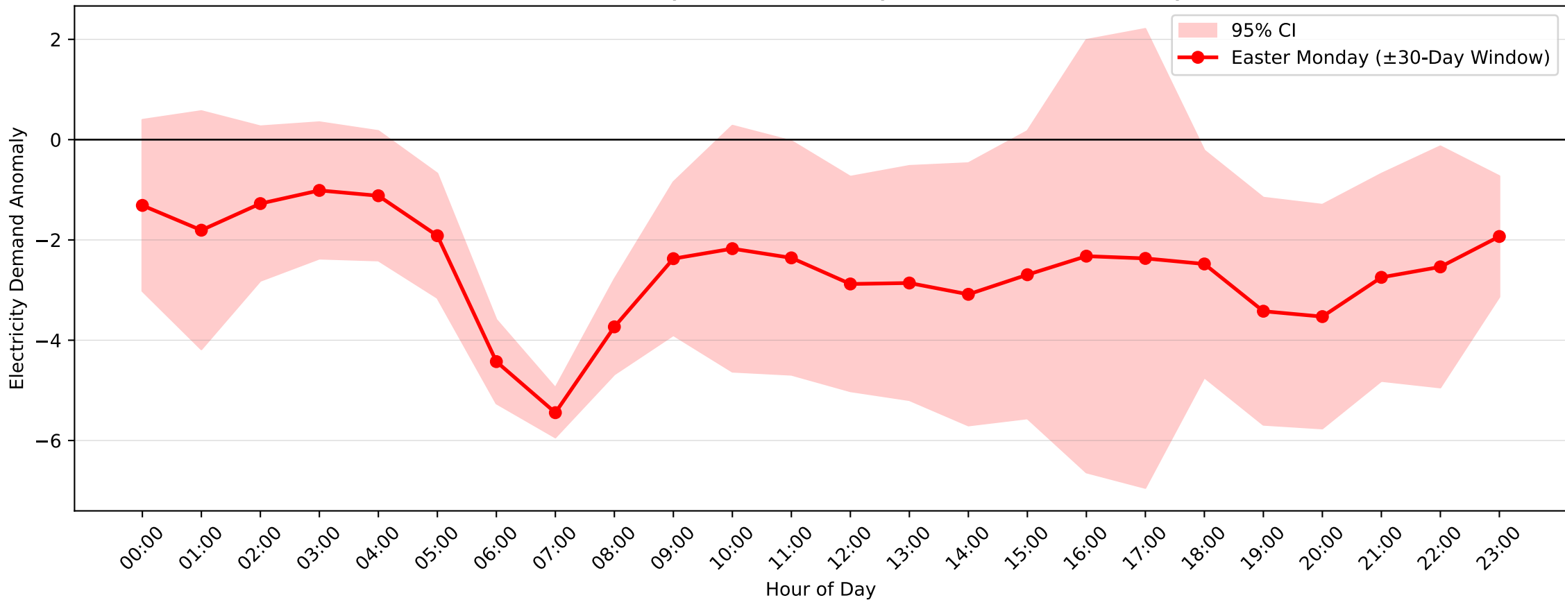
Mortdale Demand Anomaly: Easter Monday (2009–2010, \pm 30 -Day Window)
