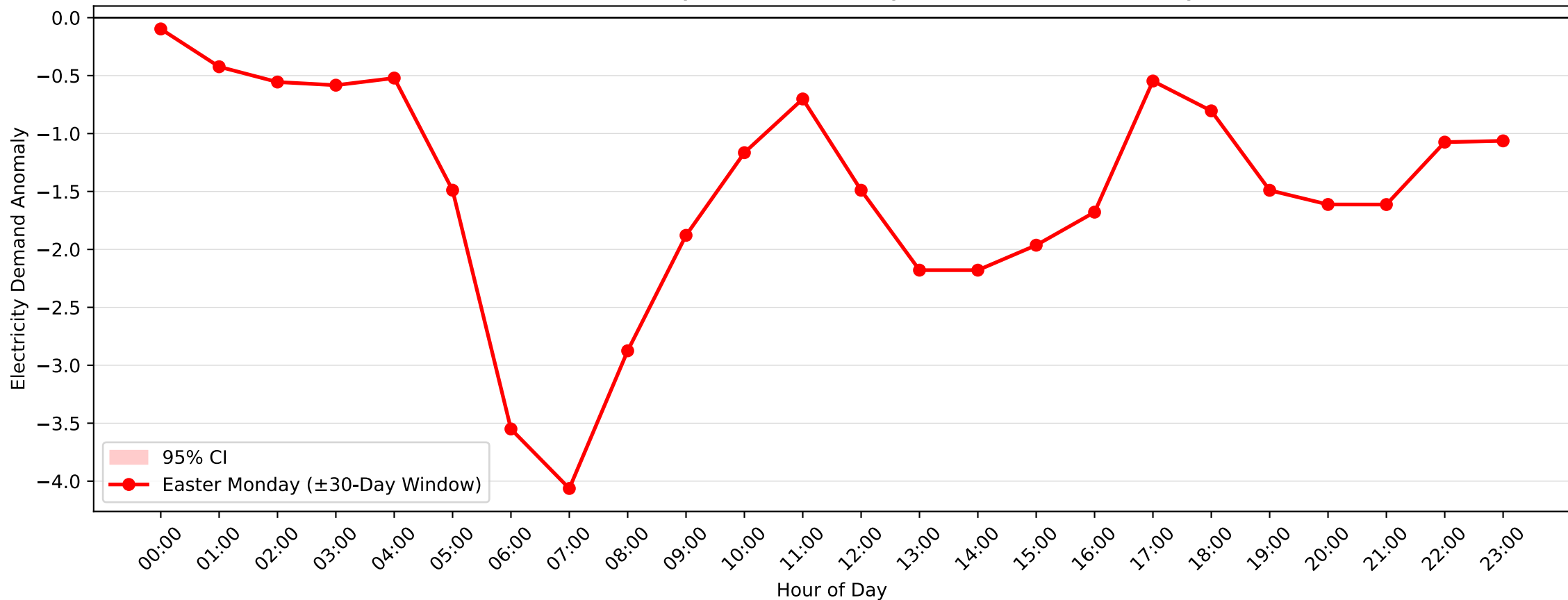
Mortdale Demand Anomaly: Easter Monday (2017-2018, \pm 30 -Day Window)
